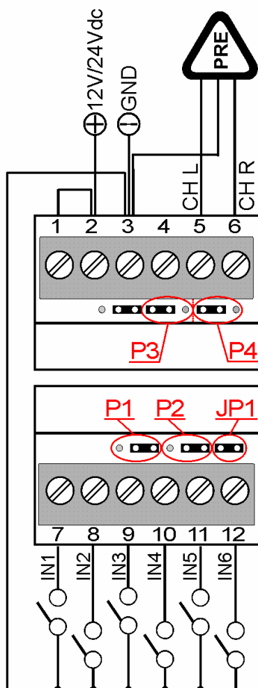
6 logical inputs and preamplified STEREO output (DEFAULT)
