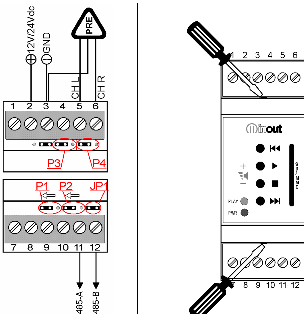
RS485 and preamplified STEREO output
