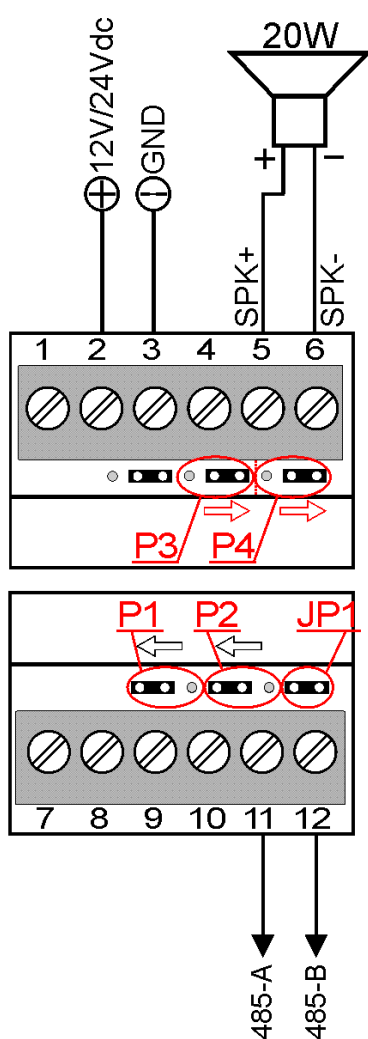
RS485 and amplified MONO output.
